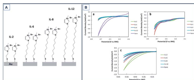
Fig. 7 Schematic of Au electrodes with 1-methylimidazolium-terminated SAMs (IL-2, IL-6, IL-8, IL-12). CV of bare and SAM modified Au electrodes in \text{Na}_2\text{SO}_4 aqueous solution purged with (a) \text{N}_2 and (b) \text{CO}_2 . Scan rate: 100 \text{ mV s}^{-1} ; (c) CV of bare and SAM-modified Au electrodes in \text{NaHCO}_3 aqueous solution purged with \text{CO}_2 . Scan rate: 100 \text{ mV s}^{-1} . 135 Copyright (2015) Royal Society of Chemistry.
