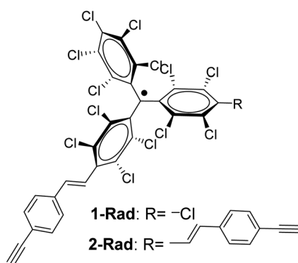
Fig. 1 Chemical structure of the PTM radicals employed in this work.
