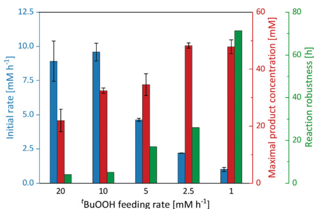
Fig. 3 Initial rate, maximal product concentration and reaction robustness of the epoxidation of \text{cis-}\beta -methylstyrene catalysed by imm- \text{rAaeUPO} at different \text{'BuOOH} feeding rates. Reaction set-up: 570 \mu\text{L} \text{cis-}\beta -methylstyrene, supplemented with 180 \text{ mg} immobilisate and continuously fed with the indicated \text{'BuOOH} rate. General reaction conditions: [\text{rAaeUPO}] = 0.5 \mu\text{M} , room temperature, shaking at 99 \text{ rpm} with 60^\circ angle in an overhead rotator. Data represents the average of duplicates.
