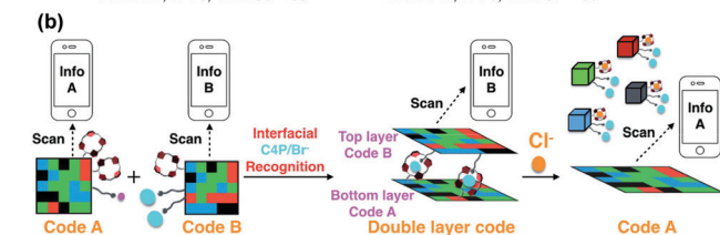
Fig. 32 (a) Chemical structures of the polymeric gels, the incorporated fluorescent elements, and the recognition elements present in Code A ( 209–212 ) and Code B ( 213–216 ). (b) The mechanism of forming a double layer code and specific sensing of Cl − anions.
