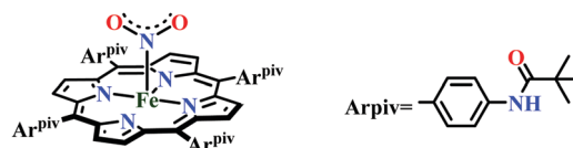
Fig. 15 Molecular structure [(TpipPP)Fe(NO 2 )] − .
