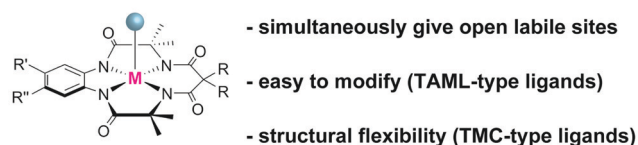
Chart 9 Summary of features of water oxidation catalysts with macrocyclic ligands.
