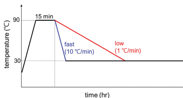
Fig. 1 A temperature control profile for polymer crystallization during the experiment.
