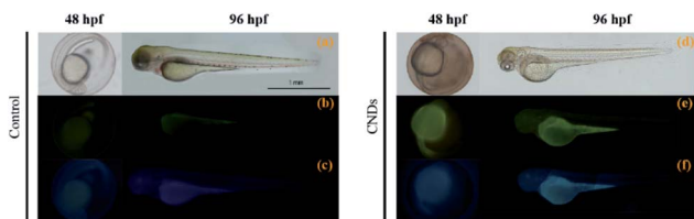
Fig. 10 Fluorescent images of zebrafish embryos (48 hpf) and larvae (96 hpf) after exposure to CNDs solution (400 mg L -1 , right panel), in comparison with control group (autofluorescence signal, left panel). (a and d) Bright field; (b and e) green fluorescent field; (c and f) blue fluorescent field.
