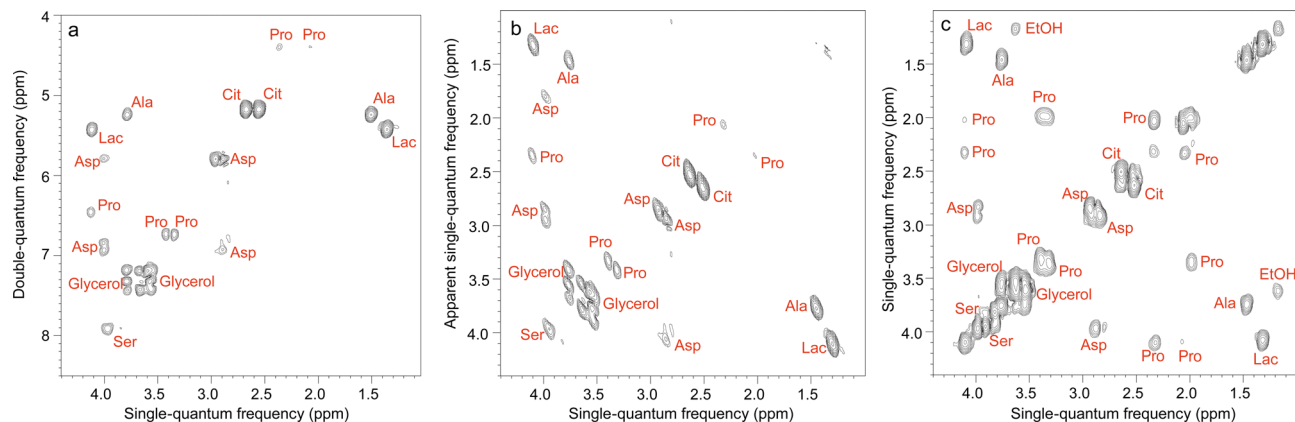
Fig. 7 Ultrafast NMR spectra of a mixture of 7 metabolites in \text{H}_2\text{O}/\text{D}_2\text{O} (90/10): (a) DQF (c) COSY. All spectra were recorded in four interleaved scans to increase the observable spectral width, and four dummy scans resulting in an acquisition time of 41 s, using a double-quantum build-up delay \tau = 25 ms. Spectrum (b) was obtained from spectrum (a) by a shearing transformation at a processing stage. All spectra were recorded with a 600 MHz spectrometer equipped with a cryogenic probe. Reproduced from ref. 156 with permission from the Royal Society of Chemistry.
