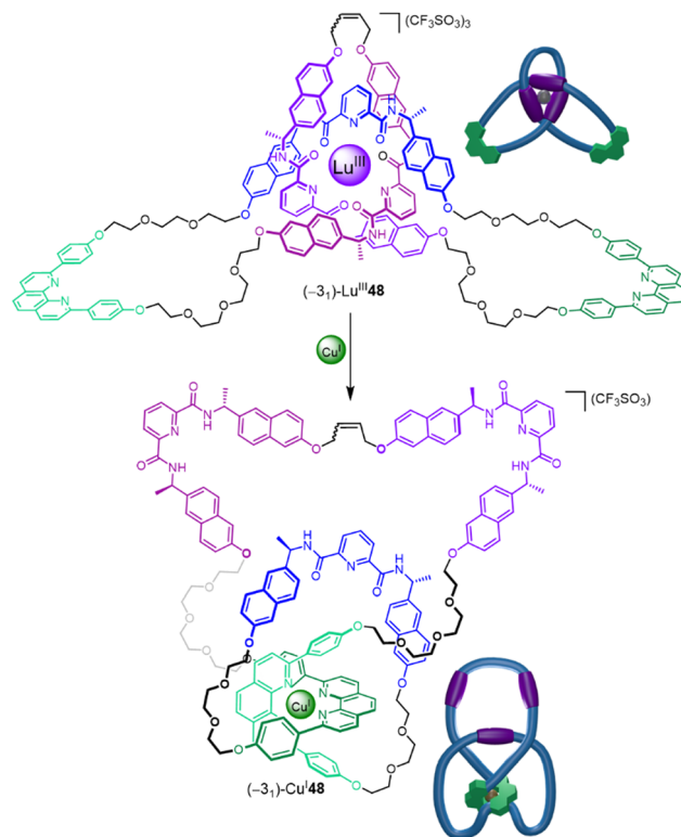
Fig. 31 Binding different metal ions changes the position of an entanglement within molecular knot (-3_1)\text{-48} . 21
