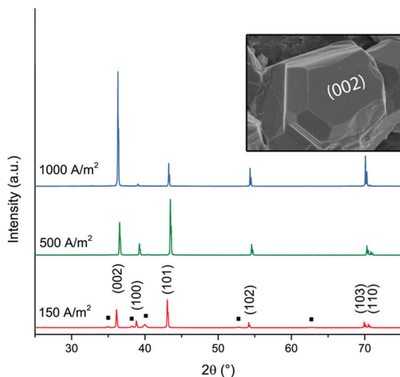
Fig. 3 XRD diffractograms of zinc deposited at current densities of 150 A m -2 , 500 A m -2 and 1000 A m -2 . The peaks corresponding to the titanium phase (JCPDS-ICDD, 44-1294) are labelled with a black square (■). The hexagonal prism analogous to the zinc crystal in Fig. 1f illustrates the corresponding directions of the crystal planes (002) and (100).
