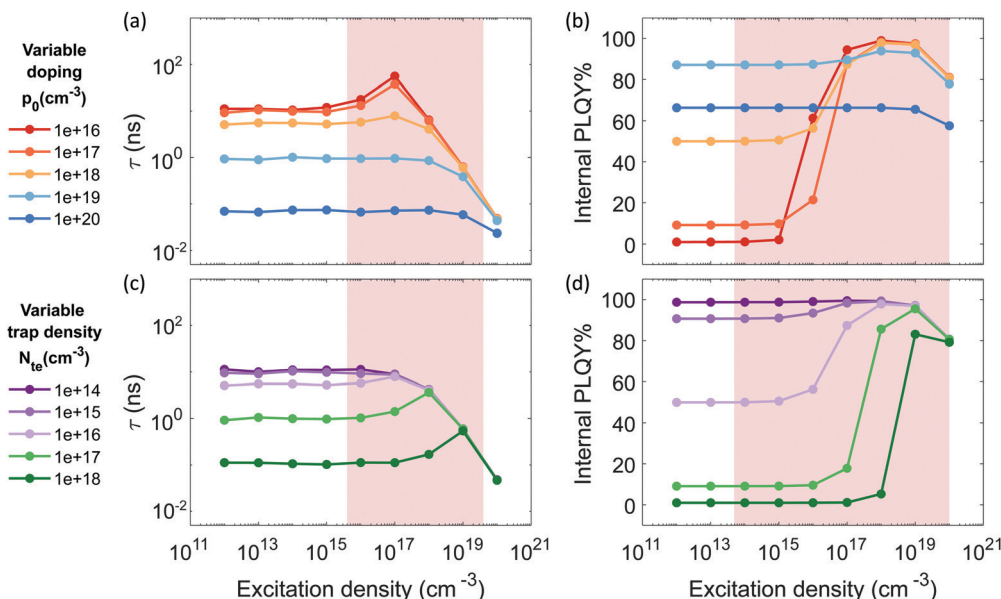
Fig. 1 Simulated carrier lifetime (a and c) and internal PLQY (b and d) as solutions to the system of equations eqn (1)–(5). (a and b) With variable doping density and trap density fixed at 10^{16} cm ^{-3} (parameters listed in Table S1 (ESI ^{\dagger} )); (c and d) with variable trap density and doping density fixed at 10^{18} cm ^{-3} (parameters listed in Table S2 (ESI ^{\dagger} )). Shaded regions indicate the experimental measurement ranges showed in Fig. 2 and 3.
