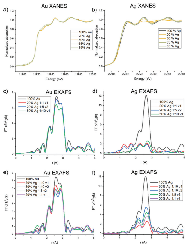
Fig. 5 Au XANES (a) shows \text{Au}^0 with altered potential at high Ag incorporation. Ag XANES (b) reveals \text{Ag}^+ character for 20 atomic % solution Ag samples, suggesting a lack of incorporation into the bulk. (c) and (d) reveal Au that shows evidence of primarily Au–Au coordination and Ag that exhibits underincorporation for the low Ag incorporation samples shown. (e) and (f) reveal differences in atomic scale coordination for samples with similar atomic % Ag, but different reductant ratios and volumes.
