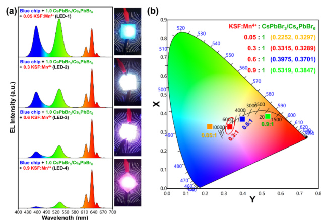
Fig. 9 (a) The electroluminescence spectra of the designed LED devices by varying the K 2 SiF 6 :Mn 4+ to CsPbBr 3 /Cs 4 PbBr 6 ratio in the wt% of 0.05 : 1, 0.3 : 1, 0.6 : 1, and 0.9 : 1 under forward-bias current of 20 mA (inset images are photographs of the working LEDs (LED 1–4)), (b) the CIE chromaticity coordinates corresponding to the constructed LED devices using different composite wt% ratios.
