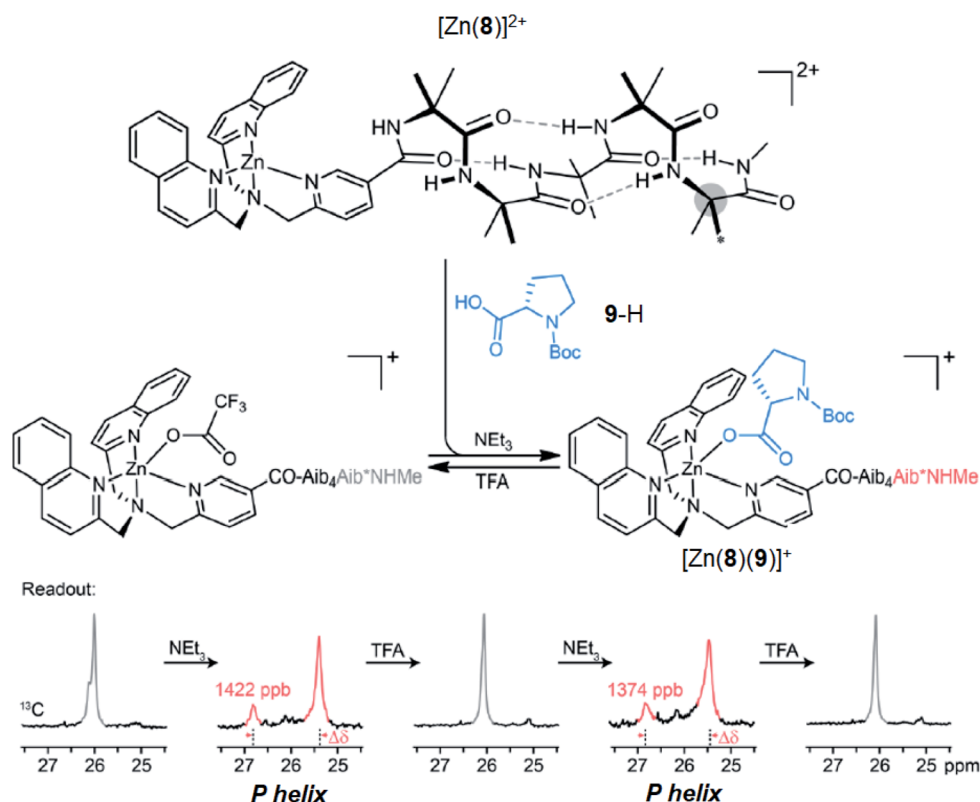
Fig. 10 pH-induced binding of 9-H with complex [\text{Zn}(\mathbf{8})]^{2+} ( c_0 = 12.1 \text{ mM} ) with alternating addition of NEt 3 and TFA in 1.2 eq. increments, monitored by 13 C NMR of the terminal Aib*NHMe reporter.
