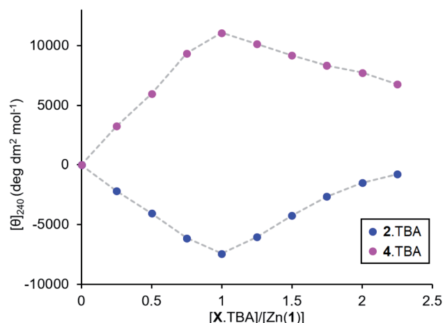
Fig. 5 Molar ellipticities at 240 nm for \text{Zn}(\mathbf{1}) \cdot 2\text{ClO}_4 ( c_0 = 0.25 mM) in MeCN with addition of 2.TBA or 4.TBA (0 \rightarrow 2.25 eq.).
