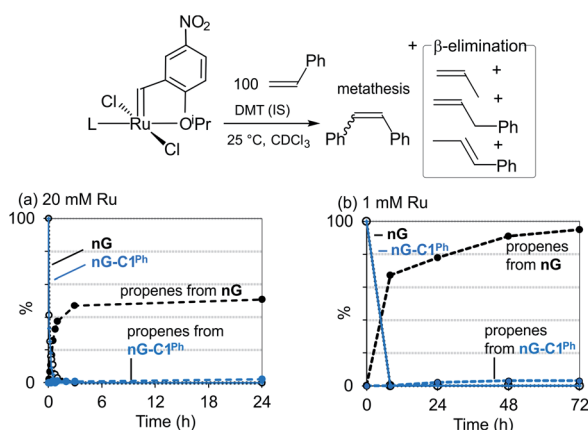
Fig. 1 Decomposition of nG and nG-C1 Ph via \beta -H elimination: disappearance of NMR signals for [Ru] = CHAr , and appearance of signals for propenes. (a) At 20 mM Ru (300 MHz). (b) At 1 mM Ru (500 MHz).
