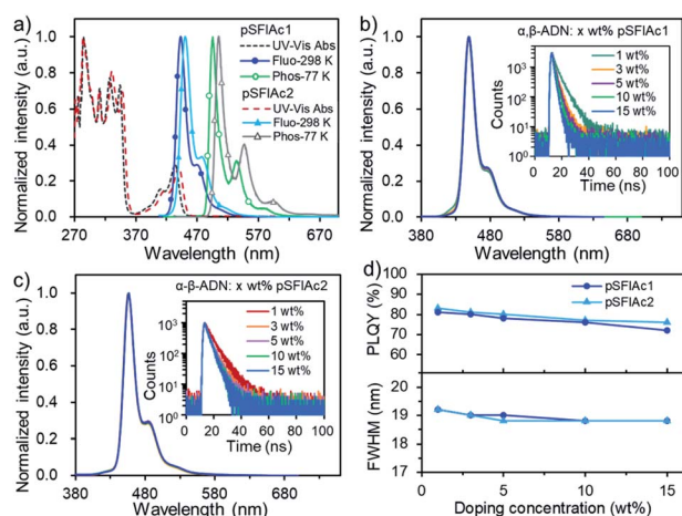
Fig. 2 (a) The absorption (left axis), fluorescence and phosphorescence (right axis) spectra of pSFIAC1 and pSFIAC2 in toluene ( 10^{-5} M). (b) and (c) The PL spectra and transient PL (inset) curves with different concentrations in \alpha,\beta -ADN: x wt% MR emitters ( x = 1, 3, 5, 10, 15). (d) The PLQYs and FWHMs of the doped films with different concentrations in \alpha,\beta -ADN: x wt% MR emitters ( x = 1, 3, 5, 10, 15).
