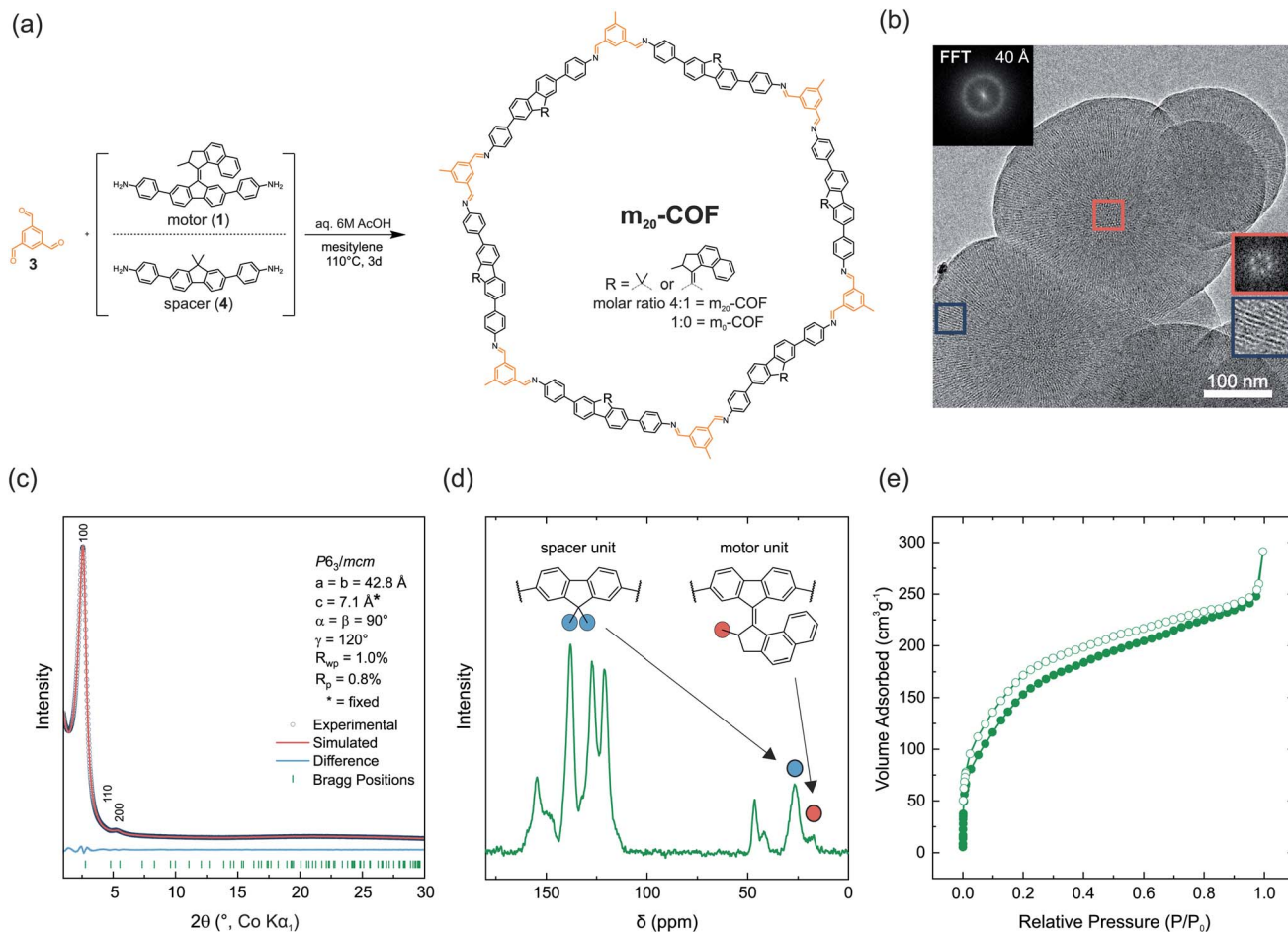
Fig. 2 (a) Synthesis of \text{m}_{20}\text{-COF} from mixtures of spacer and motor building blocks with triformylbenzene (3) under solvothermal conditions. (b) Transmission electron microscopy (TEM) image of \text{m}_{20}\text{-COF} with visible pore channels along [00l] pointing towards the surface of the spherical particle (blue inset). Fast Fourier transformed (FFT) insets show a hexagonal pattern (red box, viewing direction [00l]). (c) XRPD pattern and unit cell parameters of \text{m}_{20}\text{-COF} obtained by Pawley refinement with a simplified unit cell proxy model (see Table S1†). (d) ^{13}\text{C} -CPMAS ssNMR spectrum of \text{m}_{20}\text{-COF} containing signals of the motor and spacer building blocks. (e) \text{N}_2 adsorption isotherm of \text{m}_{20}\text{-COF} .
