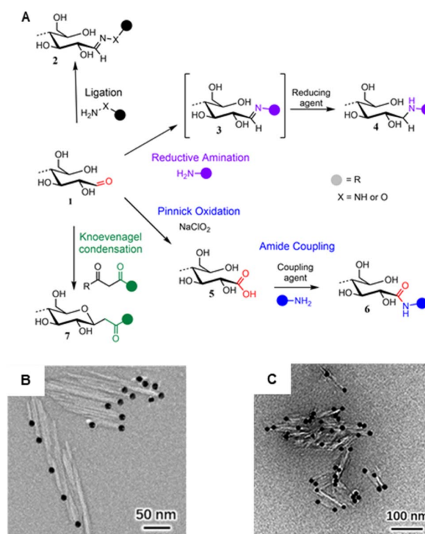
Fig. 8 (A) Main mechanisms used to target cellulose REGs (1): Ligation of hydrazine ( \text{NH}_2-\text{NH}-\text{R} ) or hydroxyl amine derivatives ( \text{NH}_2-\text{O}-\text{R} ) affording hydrazones or oximes (2); reductive amination forming an imine intermediate (3) that is reduced to a stable secondary amine (4); Pinnick oxidation affording carboxylated REGs (5) that allow for subsequent amidation (6); Knoevenagel condensation affording a C-glycoside ketone (7). (B) Asymmetric thioureation of the reducing ends of CNCs during which the aldehyde groups are converted into imine groups, and TEM images of CNC (left) and CNC-II (right) are modified with gold nanoparticles. (A) was adapted with permission from Heise et al. 165 under CC BY 4.0. Copyright 2020 Wiley. (B) was reprinted from Lin et al. , 166 Copyright 2021, with permission from Elsevier. (C) was reproduced from Lin et al. 167 with permission from Royal Society of Chemistry.
