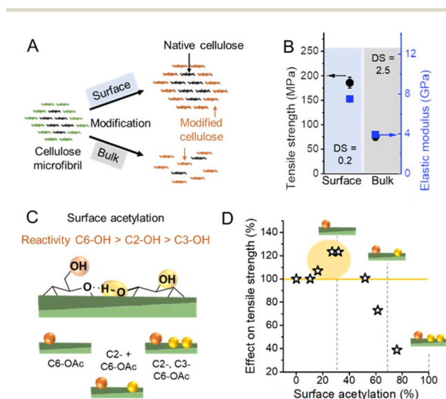
Fig. 4 (A) Schematic representation of a surface vs. bulk modification. The microfibril consists of chemically accessible surface chains (green color) and inaccessible chains in the core (black). Surface modification is confined to the surface, whereas bulk modification also affects the cellulose chains in the non-accessible, more crystalline core causing ultimately an alteration of the microfibril structure at a high degree of substitution. (B) Influence on mechanical properties of surface 53 vs. bulk acetylation. 54 (C) Possible combination of acetyl group substitution patterns at the surface of cellulose. (D) Influences of the extent of surface acetylation on the mechanical properties of cellulose. Plot B was drawn from literature data by Beaumont et al. 53 and Cindradewi et al. 54 and Plot D from data by Aiken et al. 47
