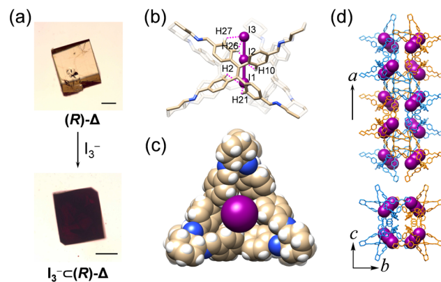
Fig. 5 Anion recognition in (R)-Δ. (a) Photographs of single crystals of (R)-Δ and [I 3 - ](R)-Δ. Scale bars represent 200 μm. (b and c) Superstructure of [I 3 - ](R)-Δ in tubular and (c) space-filling representations exhibiting the encapsulation of I 3 - inside the cavity of (R)-Δ by 18 [C–H...I] interactions. C, tan; N, blue; H, white; I, purple. (d) Side-on (top) and top (down) views of the double helical superstructure of [I 3 - ](R)-Δ. Hydrogen atoms are omitted for clarity. One strand in the double helix is depicted in orange tubular representation and the other in blue, while I 3 - is represented in a space-filling form.
