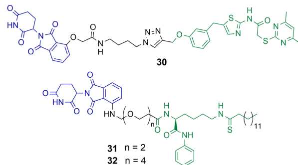
Chart 6 PROTACs reported for the selective degradation of SIRT2. 30 degrades SIRT2 selectively over SIRT 1 at a concentration range of 0.2–10 \mu\text{M} in HeLa cells. 49 31 and 32 degrade SIRT2 at concentration range of 0.5–10 \mu\text{M} in MCF7 and BT-549 cells with no SIRT1 degradation observed. 85
