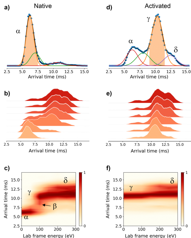
Fig. 2 Multistage cyclic IM-MS experiments. Arrival time distribution (ATD) recorded for the mass-selected \text{Zn}_7\text{MT}_2^{5+} ions ( 1298\text{ m/z} ) under non-activating conditions (a) and activated on injection to the trap prior to IM selection (d). The IMS-CA-IMS and CA-IMS-CA-IMS approach in which the conformer \alpha (b) and conformer \gamma (e) were isolated and reinjected from the pre-store into the array at increasing activation energies, respectively. Unfolding profiles for the IMS-CA-IMS (c) and CA-IMS-CA-IMS approach (f).
