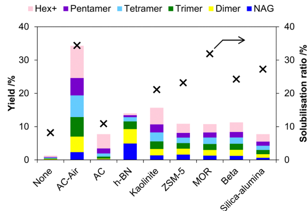
Fig. 10 Screening of solid catalysts in the mechanochemical hydrolysis of chitin. Hex+ indicates the total yield of hexamer and larger oligomers. Yield is based on moles of carbon.
