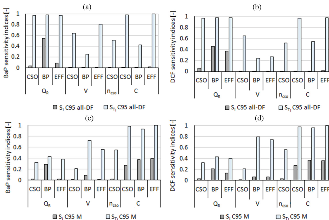
Fig. 7 S_1 (in grey) and S_{1i} (in light blue) values for (a) BaP and (b) DCF in the all-DF scenario; in the medium scenario for (c) BaP and (d) DCF. Results refer to the scenario using the C95 distribution.
