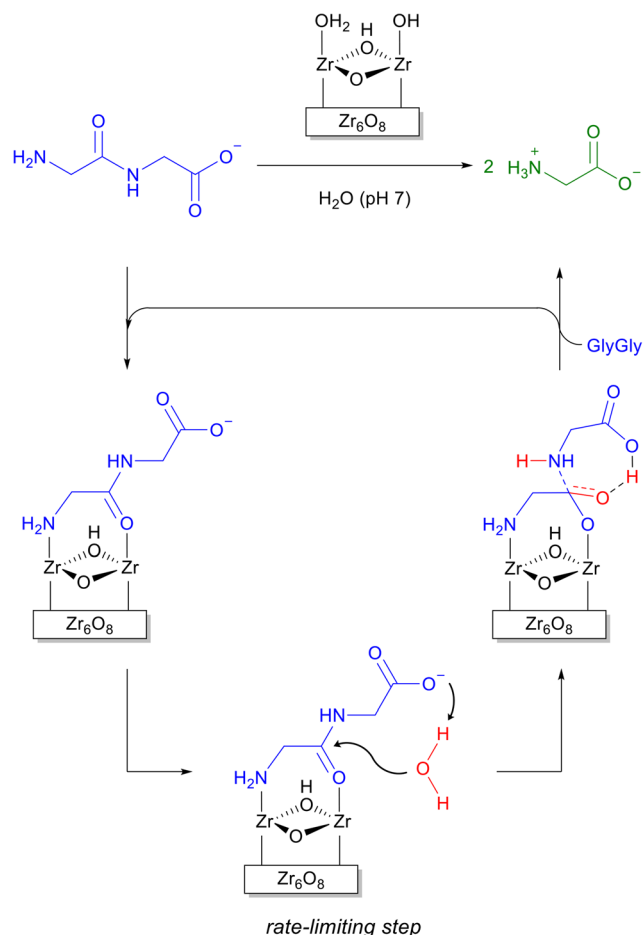
Scheme 1 General mechanism of peptide bond hydrolysis at the Zr_6O_8 cluster nodes of Zr-MOFs.
