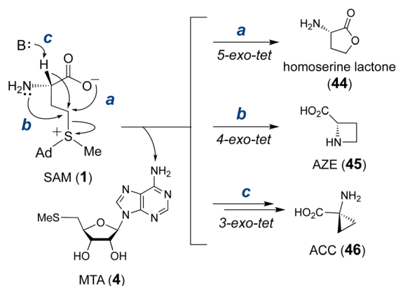
Fig. 12 Intramolecular cyclization of the SAM aminocarboxypropyl moiety into homoserine lactone ( 44 , via route a), azetidine 2-carboxylic acid (AZE, 45 , via route b) and 1-aminocyclopropane-1-carboxylic acid (ACC, 46 , via route c), each with elimination of MTA ( 4 ).
