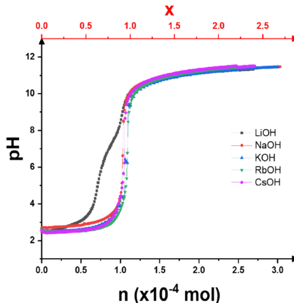
Fig. 1 Potentiometric titration curves of \text{H}_3\text{Sb}_3\text{P}_2\text{O}_{14} dispersions with different alkaline base solutions: \text{LiOH} , \text{NaOH} , \text{KOH} , \text{RbOH} , and \text{CsOH} . x (top axis) is the theoretical exchange rate.
