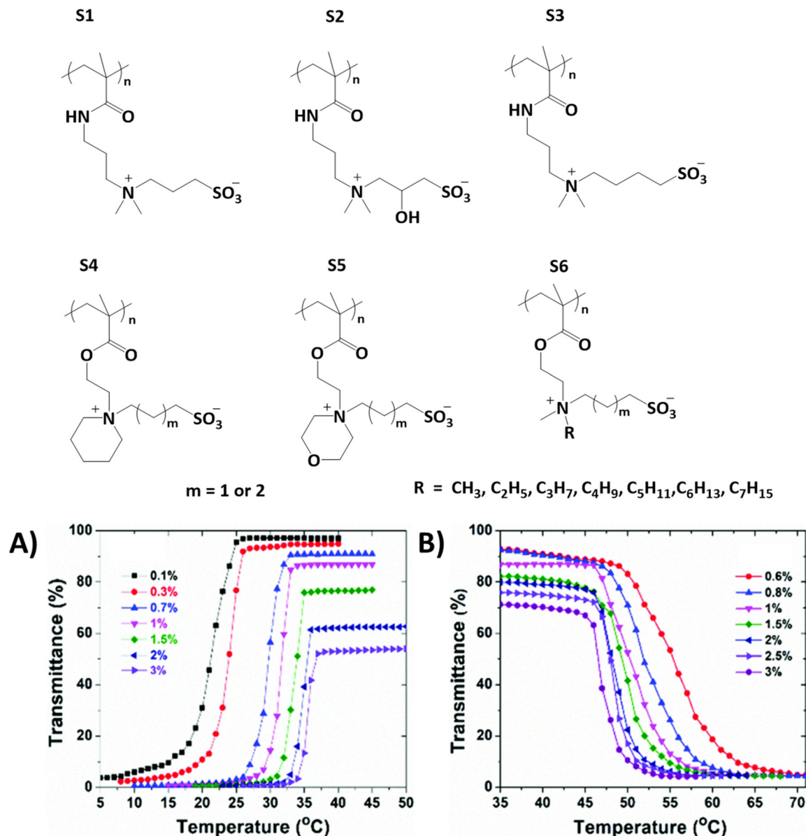
Fig. 2 Series of zwitterionic polysulfobetaines. (A) Transmittance data collected upon cooling S6 with methyl substituents; (B) collected upon heating S6 with an n -pentyl substituent at various polymer concentrations. Reproduced from ref. 64. Copyright 2018 Royal Society of Chemistry.
