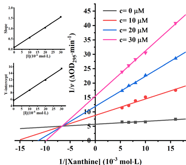
Fig. 3 Lineweaver–Burk plots. c(\text{XO}) = 0.025 \text{ U mL}^{-1} , c(\text{AUR}) = 0, 10, 20 and 30 \text{ }\mu\text{M} ; the secondary plot represented slope and Y-intercept vs. [\text{AUR}] in the inset, respectively.
