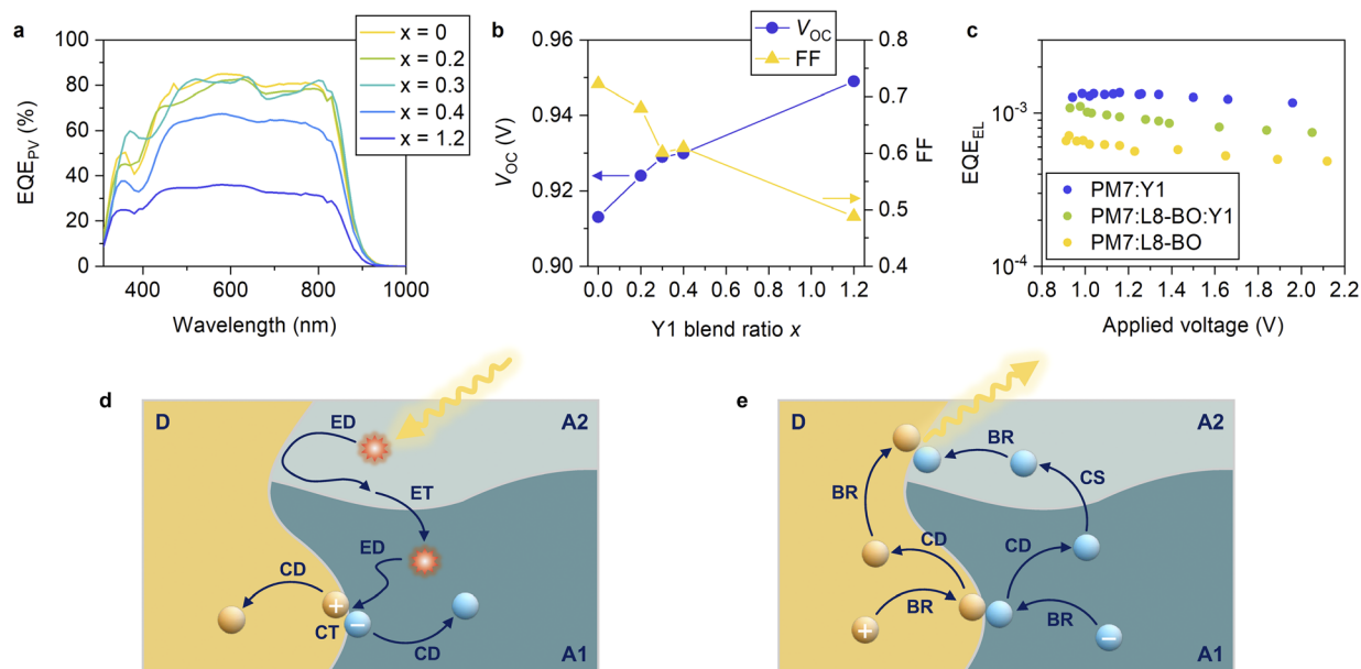
Fig. 7 (a) \text{EQE}_{\text{PV}} spectra of PBDB-T-2Cl:L8-BO:Y1 ternary blend devices with different blend ratios. The blend ratios were varied over 1:1.2- x : x , as indicated in the figure. (b) Blend ratio dependence of V_{\text{OC}} (blue circles, left axis) and FF (yellow triangles, right axis). (c) \text{EQE}_{\text{EL}} of the PBDB-T-2Cl:L8-BO:Y1 (1:1:0.2) ternary blend device as well as its binary references. (d) Schematic showing the charge separation process. Hole transfer is slow at the donor:minority NFA (D:A2) interface, and the CT states are not likely to form. On the other hand, excitons can move between the majority and minority NFA domains without a large energetic barrier. Therefore, charge separation preferentially occurs at the donor:majority NFA (D:A1) interface following exciton (energy) transfer from the minority to majority NFAs. ED, ET, CT, and CD refer to exciton diffusion, energy (exciton) transfer, charge transfer, and charge dissociation, respectively. (e) Schematic showing the charge recombination process. Because the redissociation of the CT state is less efficient at the D:A2 interface compared to that at the D:A1 interface, charge recombination is expected to be more likely to occur at the former. Because the \text{EQE}_{\text{EL}} of the D:A2 blend is higher than that of the D:A1 blend, the preferential recombination at the former leads to an increase in the \text{EQE}_{\text{EL}} of the ternary blend. BR and CS refer to bimolecular charge recombination to regenerate the CT states, and charge shift between A1 and A2, respectively.
