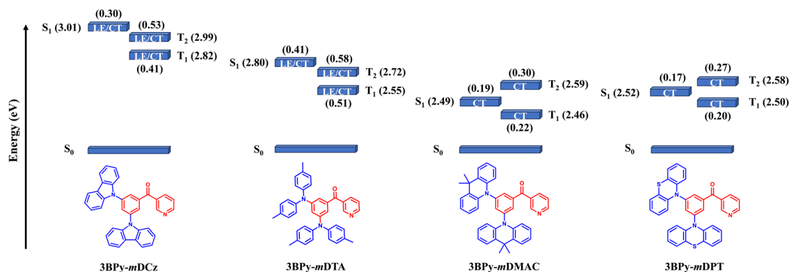
Fig. 6 Energy level diagram of excited states ( S_1 , T_1 and T_2 ) for 3BPY-mDCz , 3BPY-mDTA , 3BPY-mDMAC and 3BPY-mDPT where the value in brackets indicates the hole–electron overlap for the specified level.
