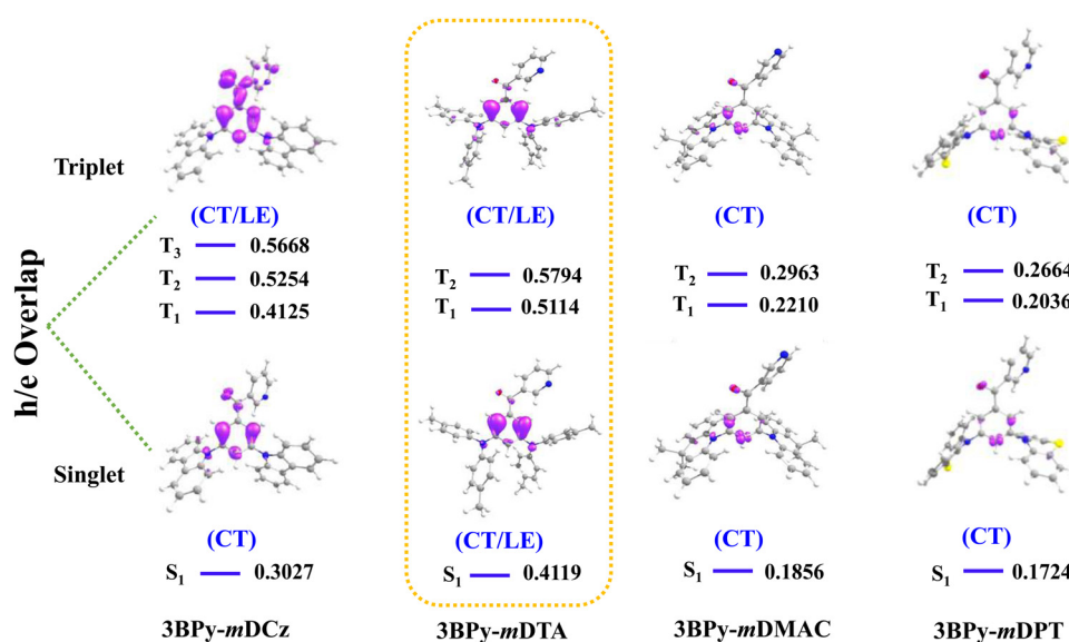
Fig. 7 Hole and electron overlap (h/e) in the singlet and triplet excited state of 3BPY-mDCz , 3BPY-mDTA , 3BPY-mDMAC and 3BPY-mDPT , respectively, with the corresponding obtained energy state.
