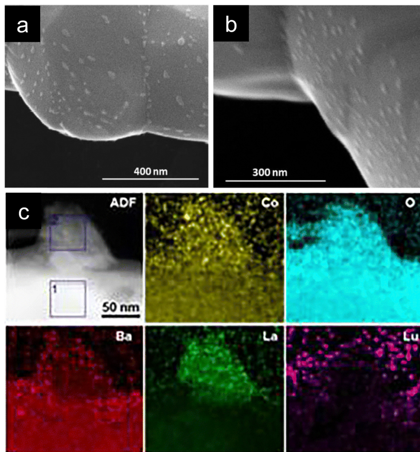
Fig. 4 (a) and (b) SEM micrographs of \text{Ba}_{0.5}\text{La}_{0.4}\text{Lu}_{0.1}\text{CoO}_3 depicting the oxide nanoparticle decoration over this double perovskite. (c) HAADF and EDX mappings of an exsolved nanoparticle composed of Co, La, Ba and O from \text{Ba}_{0.85}\text{La}_{0.15}\text{Co}_{0.75}\text{Lu}_{0.25}\text{O}_{3-\delta} . Reproduced from ref. 35 with permission from the Royal Society of Chemistry.
