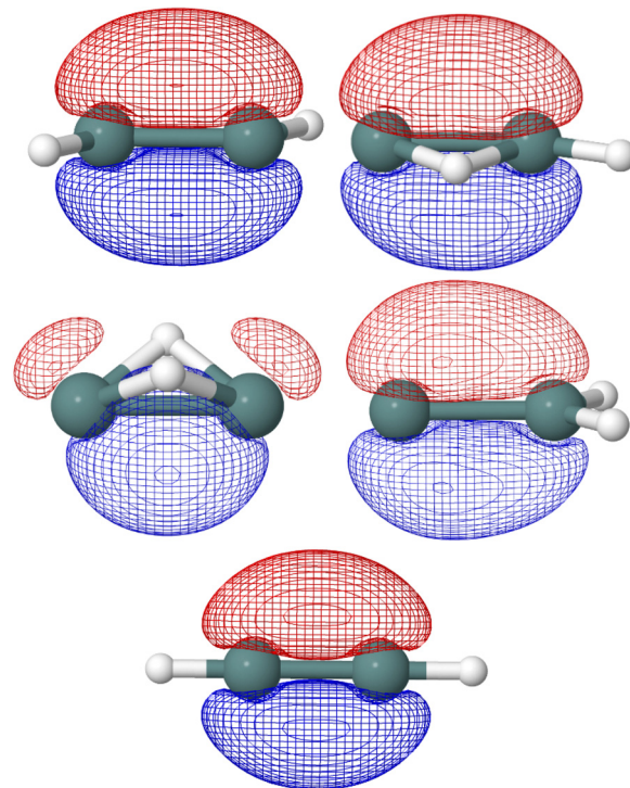
Fig. 4 HF/def2-TZVP singly-occupied molecular orbitals of the \text{Ge}_2\text{H}_2^+ structures computed at CCSD(T)/cc-pwCVQZ-PP optimized geometries are shown. From left to right and top to bottom: trans ( C_{2h} ; ^2A_u ), monobridged ( C_s ; ^2A'' ), butterfly ( C_{2v} ; ^2A_1 ), germlydene ( C_{2v} ; ^2B_2 ), and linear ( D_{\infty h} ; ^2\Pi_u ).
