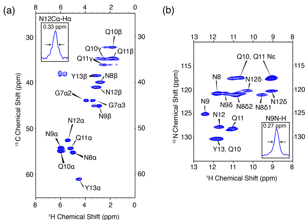
Fig. 2 High resolution ^1\text{H} detected CP-HSQC spectra of nanocrystalline \text{U-}^{13}\text{C}, ^{15}\text{N} -GNNQQNY at \omega_{\text{r}}/2\pi = 90 kHz, \omega_{\text{H}}/2\pi = 800 MHz. (a) ^1\text{H} – ^{13}\text{C} correlations. (b) ^1\text{H} – ^{15}\text{N} correlations. The mixing times and other spectral acquisition parameters are provided in Table S2 (ESI†).
