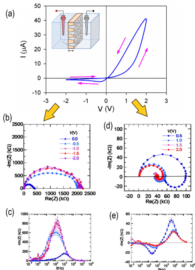
Fig. 1 (a) Current–voltage curve measured at a frequency of \Omega_s = 10 Hz for a multipore membrane in 100 mM KCl solution at a neutral pH. The inset shows the electrochemical cell with the membrane. (b) The impedance spectra at different reverse voltages, with the corresponding bode plot of the imaginary part of the impedance in (c). (d) and (e) The impedance spectra and bode plots at a forward voltage. Adapted from P. Ramirez, J. Cervera, S. Nasir, M. Ali, W. Ensinger and S. Mafe, Electrochemical impedance spectroscopy of membranes with nanofluidic conical pores, J. Colloid and Interface Sci. , 2024, 655 , 876–885, with permission from Elsevier. 29
