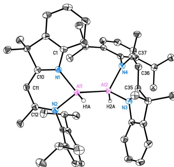
Fig. 1 Molecular structure of [(DNI(H)Al)_2] ( 2 ). The anisotropic displacement parameters are depicted at 50% probability level. All ligand-based hydrogen atoms are omitted for clarity. Selected bond lengths (Å) and angles (°): Al(1)–Al(2) 2.6007(6), Al(1)–H(1A) 1.519(12), Al(2)–H(2A) 1.528(13), Al(1)–N(1) 1.9235(11), Al(1)–N(2) 1.9407(11), Al(2)–N(3) 1.9257(11), Al(2)–N(4) 1.9391(11); N(1)–Al(1)–N(2) 93.27(5), N(3)–Al(2)–N(4) 92.60(5), H(1A)–Al(1)–Al(2) 107.6(6), H(2A)–Al(2)–Al(1) 125.0(6), C(10)–C(11)–C(12) 125.64(12), C(35)–C(36)–C(37) 125.58(11).
