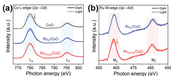
Fig. 8 (a) In situ sXAS spectra of Co L-edge for CoO, \text{Ru}_\text{O}/\text{CoO} , and \text{Ru}_{\text{O+Co}}/\text{CoO} . (b) In situ sXAS spectra of Ru M-edge for \text{Ru}_\text{O}/\text{CoO} and \text{Ru}_{\text{O+Co}}/\text{CoO} . Reprinted with permission from ref. 99. Copyright 2022 Wiley-VCH GmbH.
