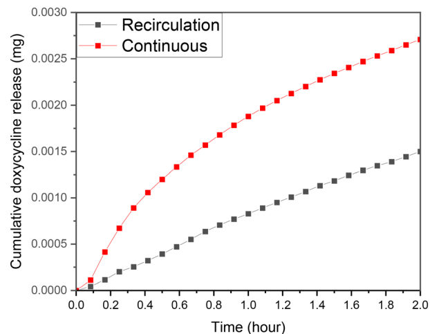
Fig. 10 Release profile for CS-2 under stimulated flow continuous flow and re-circulatory flow, pH 5.5, 37 °C cross sectional area of 7 mm 2 , depth of 0.5 mm, and 10 \mu L volume.
