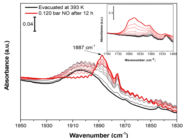
Fig. 8 IR spectra of Cu-EtP evacuated at 393\text{ K} after adsorption of 0.122\text{ bar} of NO at beam temperature and following outgassing. Black curve represents the sample evacuated at 393\text{ K} for 12\text{ h} , red curve represents 0.120\text{ bar} of NO dosed on Cu-EtP measured after 12\text{ h} and thinner coloured curves the intermediate pressures reached during outgassing. The inset reports the corresponding 1780\text{--}1480\text{ cm}^{-1} spectral region.
