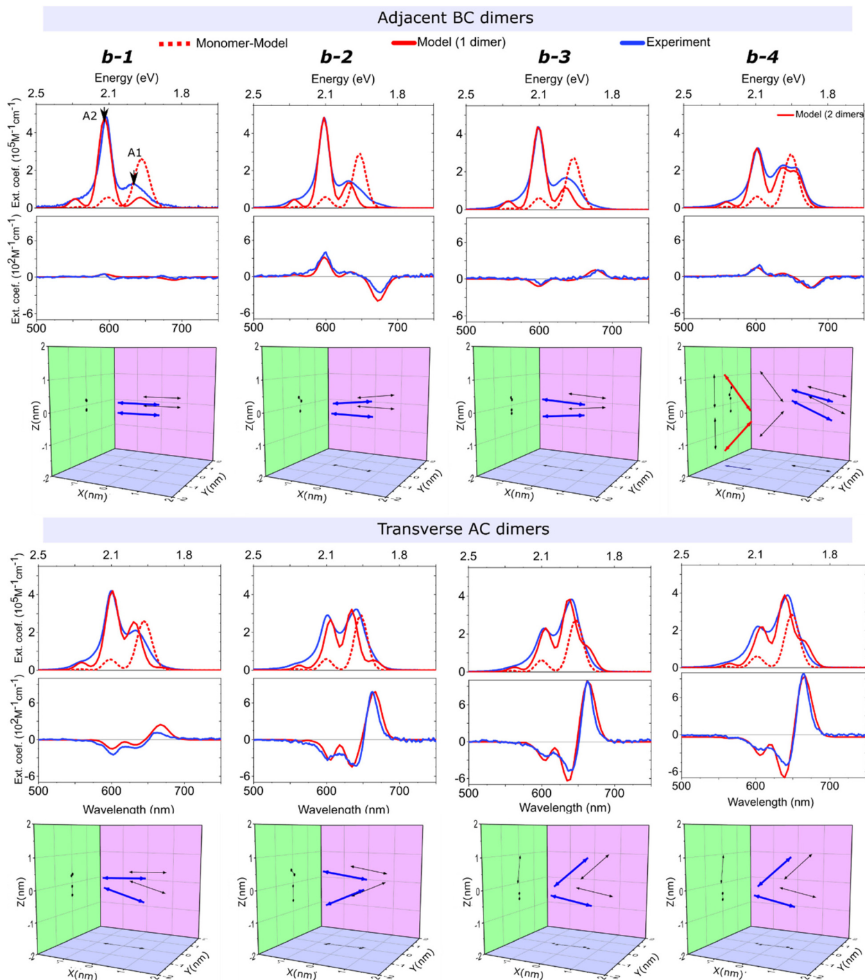
Fig. 4 Experimental and modeled absorption and circular dichroism (CD) spectra of the chlorinated squaraine dyes (plots in first and third rows). 3D plots of transition dipole moments of dyes (blue and red arrows projected to XY, YZ, and XZ planes in black arrows) derived from the KRM modeling (plot in second and fourth rows). In heterogeneous aggregates, the distance between dimers is around 1 \mu\text{m} . Experimental data (absorption and CD) of b-1 dimer was taken from our previous study. 34 "A1" indicates the low energy absorbance peak aligned with the monomer spectra, and "A2" represents the high energy absorbance peak that appears upon the formation of aggregates.
