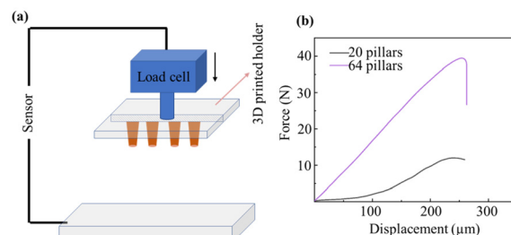
Fig. 4 A schematic of the compression force measurement and resulting force-displacement curves. (a) The compression force measurement with a maximum load cell of 50 \text{ N} , (b) force vs. displacement curves for different numbers of pillars.
