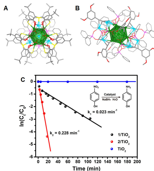
Fig. 10 Molecular structures of (A) thiacalixarene- and (B) alkynyl-protected \text{Ag}_{21} NCs. (C) Catalytic activity of \text{Ag}_{21}(\text{thiacalixarene})/\text{TiO}_2 (1/ \text{TiO}_2 ) and \text{Ag}_{21}(\text{alkynyl})/\text{TiO}_2 (2/ \text{TiO}_2 ) and \text{TiO}_2 in nitrophenol reduction. Reproduced with permission from ref. 118. Copyright (2022).
