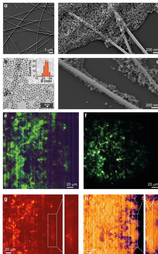
Fig. 1 (a) SEM image of AgNWs deposited on silicon wafer, (b) TEM image of UCNPs. Inset: particle size distribution. The solid line is a fit of a normal distribution. (c and d) SEM image of AgNWs on glass coated with UCNPs by drop-casting. (e) HSM image. 50 \times magnification, applied voltage = 0 V, acquisition time = 250 ms. Laser power = 0.25(2) W cm -2 . (f) Optical image under NIR (980 nm) light illumination. (g) Intensity map constructed from the integration of the UC spectra at each pixel showing enhanced emission intensity along the NWs. (h) Map of the signal-to-noise ratio calculated as described in the ESI.† The white-dashed contour highlights a single NW hardly seen in the intensity map but clearly exposed in the SNR map.
