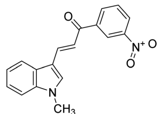
3-(1-Methyl-1H-indol-3-yl)-1-(3-nitrophenyl)prop-2-en-1-one
