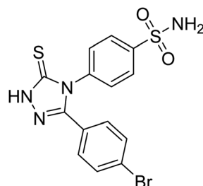
4-[3-(4-Bromophenyl)-5-thioxo-1,5-dihydro-4H-1,2,4-triazol-4-yl]benzenesulfonamide
