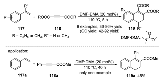
Scheme 34 Synthesis of ADHNs via DMF·DMA-catalysed cyclic addition of vinylarenes with acetylenedicarboxylate.
