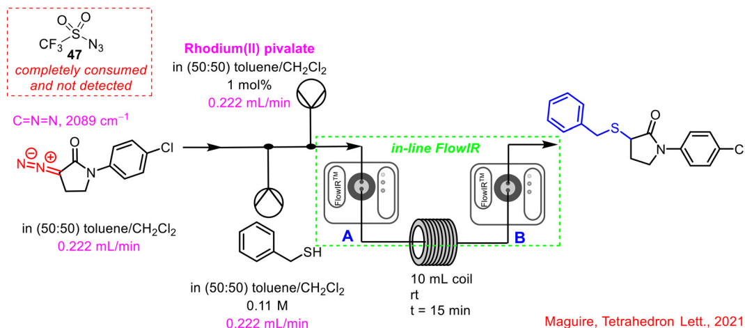
Scheme 17 Incorporation of an in-line FlowIR cell post-diazo transfer reaction and post-S-H insertion reaction by Maquire and co-workers. 57
