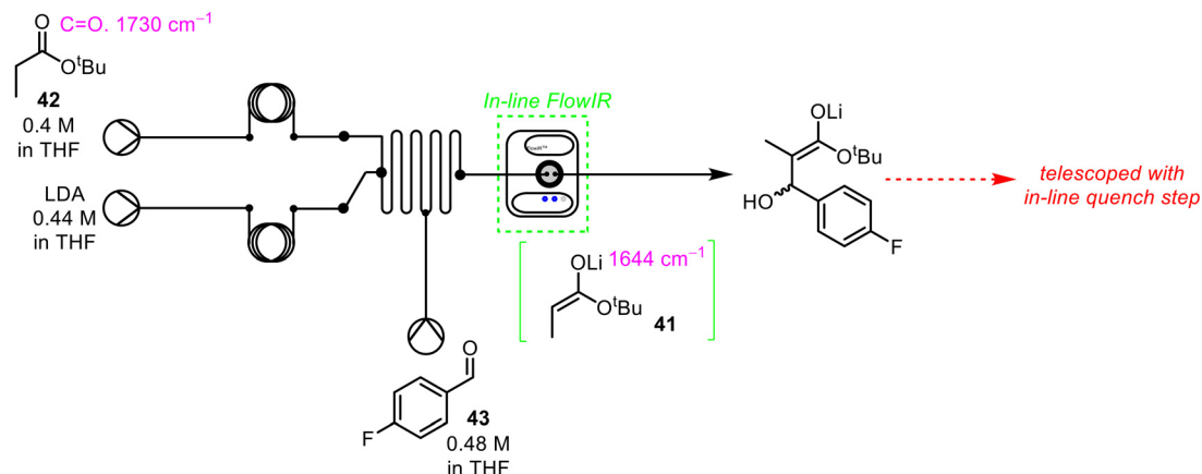
Scheme 15 Simplified schematic of in-line FlowIR cell used by Kappe and co-workers for organolithium transformation. 11
