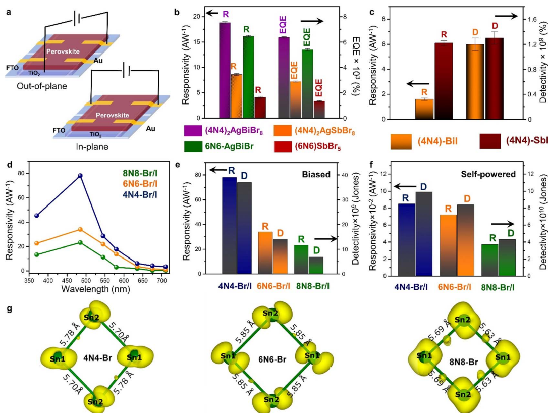
Fig. 7 (a) Schematic demonstration of the out-of-plane and in-plane photodetector devices. Statistical bar diagrams of (b) R and EQE (%) of the HLPD structures, and (c) R and D of 1D 4N4-Bil, and 4N4-Sbl. 11 (d) Wavelength dependant variation of R , and statistical bar diagram of R and D under (e) potential-biased, and (f) self-powered conditions for the DJ ( x Nx)Sn(Br/I) 4 ( x = 8N8, 6N6, 4N4 ). 23 (g) The spatially resolved charge density corresponding to the CBM of 4N4-Br, 6N6-Br, and 8N8-Br. The bond lengths of the inorganic network formed by the Sn atoms are also shown. 23 Reproduced with permission from ref. 11, copyright (2023) Royal Society of Chemistry, and ref. 23, copyright (2023) American Chemical Society of Chemistry.
