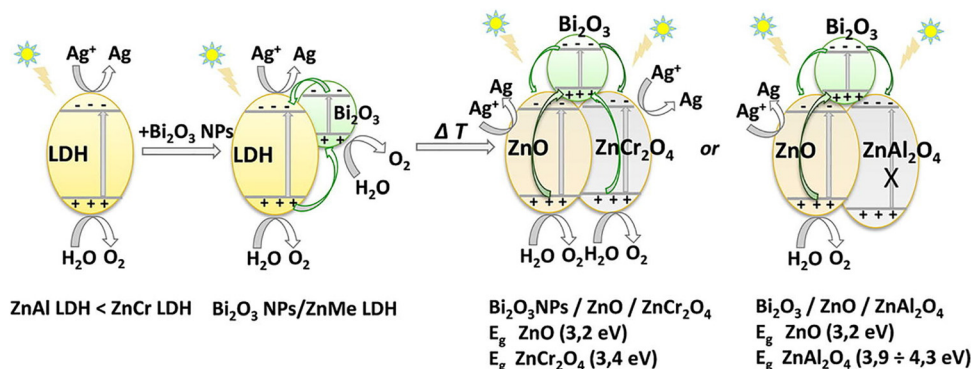
Scheme 4 Proposed mechanism for \text{O}_2 -generation under solar-light irradiation over \text{Bi}_2\text{O}_3 NPs/ZnMe-LDH and \text{Bi}_2\text{O}_3 /ZnO/ \text{ZnMe}_2\text{O}_4 .
