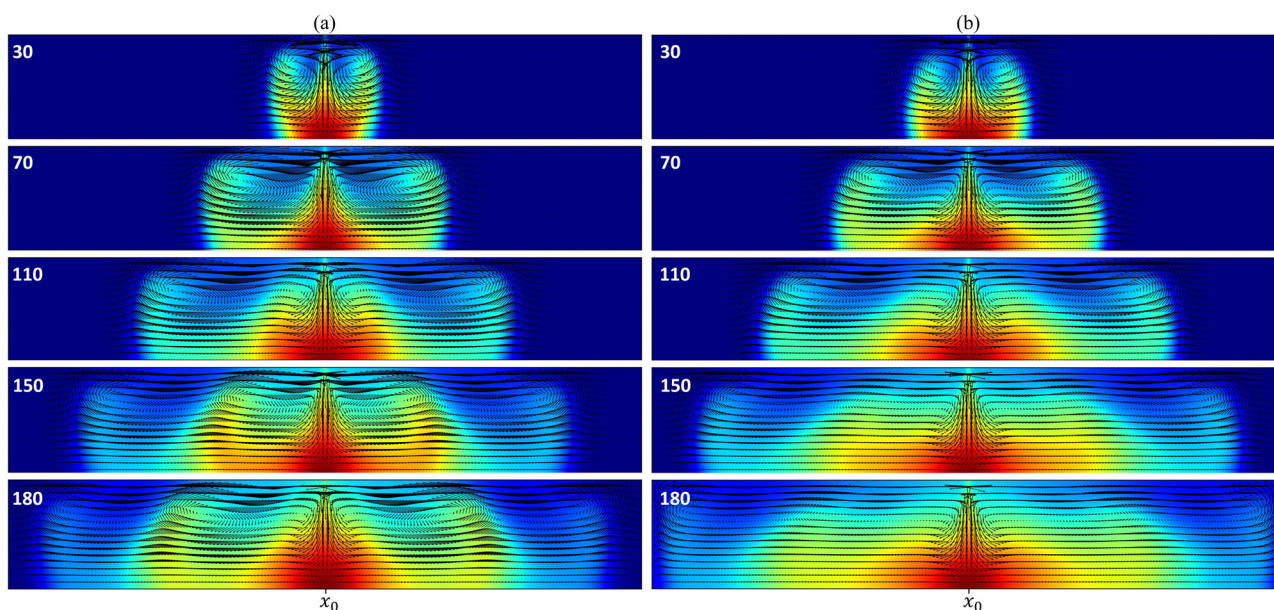
Fig. 3 Typical spatio-temporal evolution of the product concentration with increasing dimensionless time for systems of length L_x = 256 , height L_z = 20 in (a) pure Marangoni case ( \Delta M = 300 and \Delta R = 0.00 ) and (b) coupled Marangoni-buoyancy cooperative case ( \Delta M = 300 and \Delta R = -0.50 ). The fluid velocity field is superimposed on a 2D field of the product concentration c ranging from 0 (blue areas) to the highest concentration, c = 0.44 (red areas).
