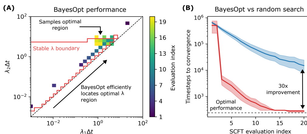
Fig. 3 Selection of relaxation coefficients \lambda = \{\lambda_1, \lambda_2\} using Bayesian optimization (BayesOpt) for SCFT of a two-species homopolymer blend. (A) BayesOpt rapidly identifies optimal regions of relaxation coefficients \lambda in fewer than 10 iterations and subsequently focuses its sampling in this region to locate the best performing \lambda . (B) Comparison of BayesOpt and random sampling. BayesOpt locates relaxation coefficients that are considerably faster than those found with random sampling. The shaded regions are 95% confidence intervals.
